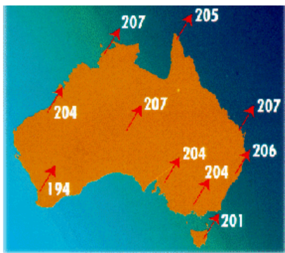
Figure 1-4: Difference between AGD and GDA94 coordinates
