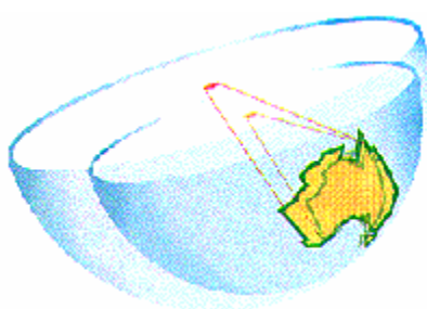
Figure 1-1: Changing datums
