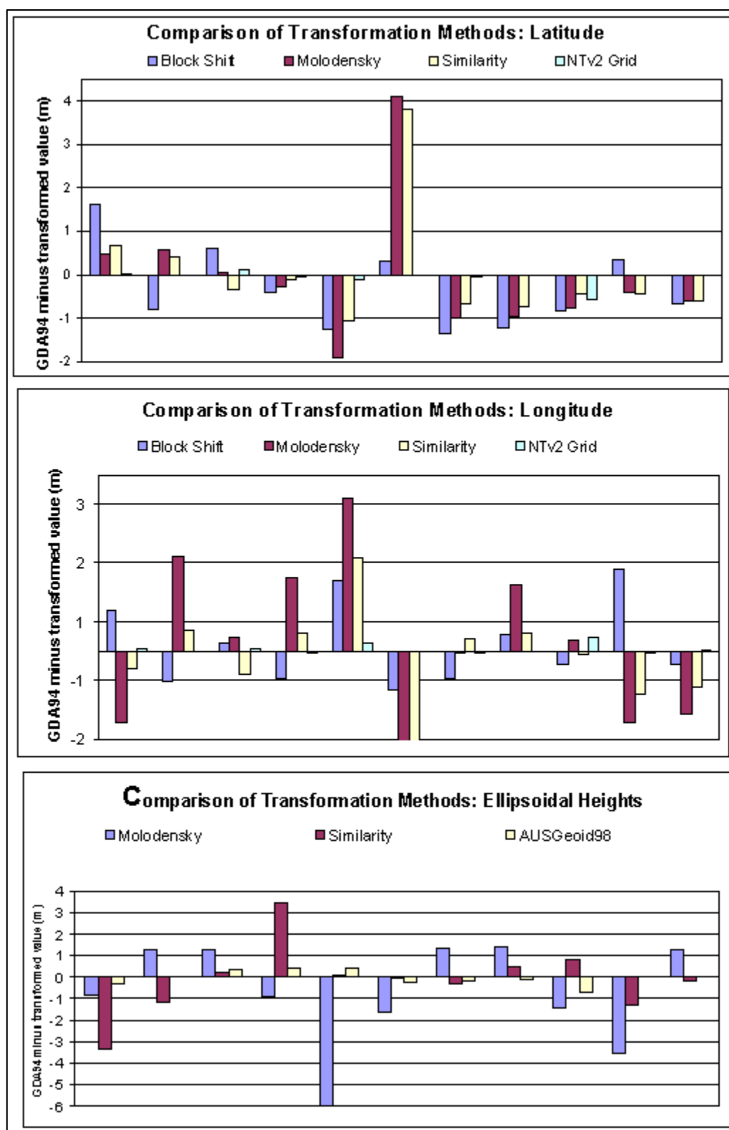
Figure 7-4: Comparison of transformation methods for latitude, longitude and height.
