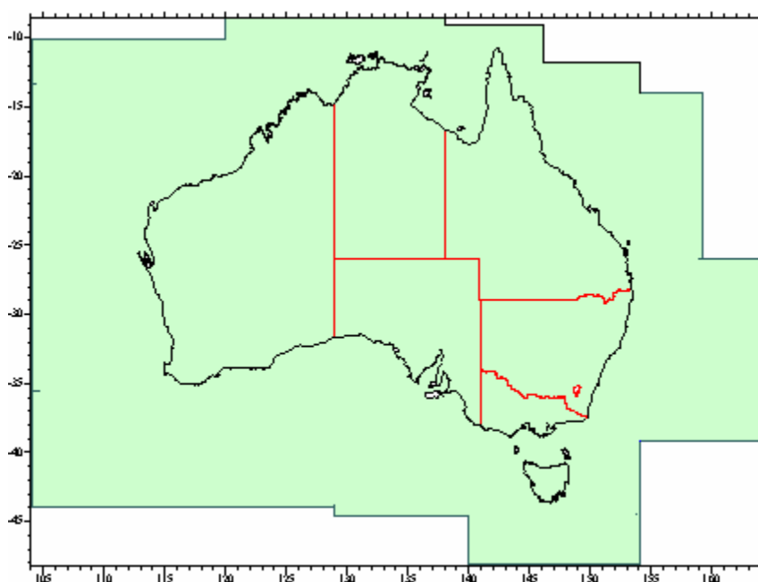
Figure 7-1 AGD66 to GDA94 Transformation Grid Coverage
