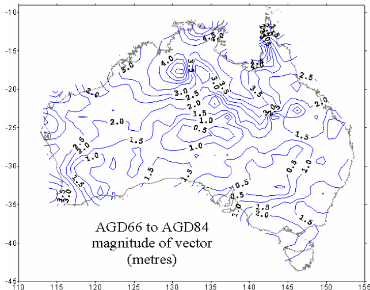
Figure 7-3: Magnitude of Block Shift vector, in metres, between AGD66 and AGD84
