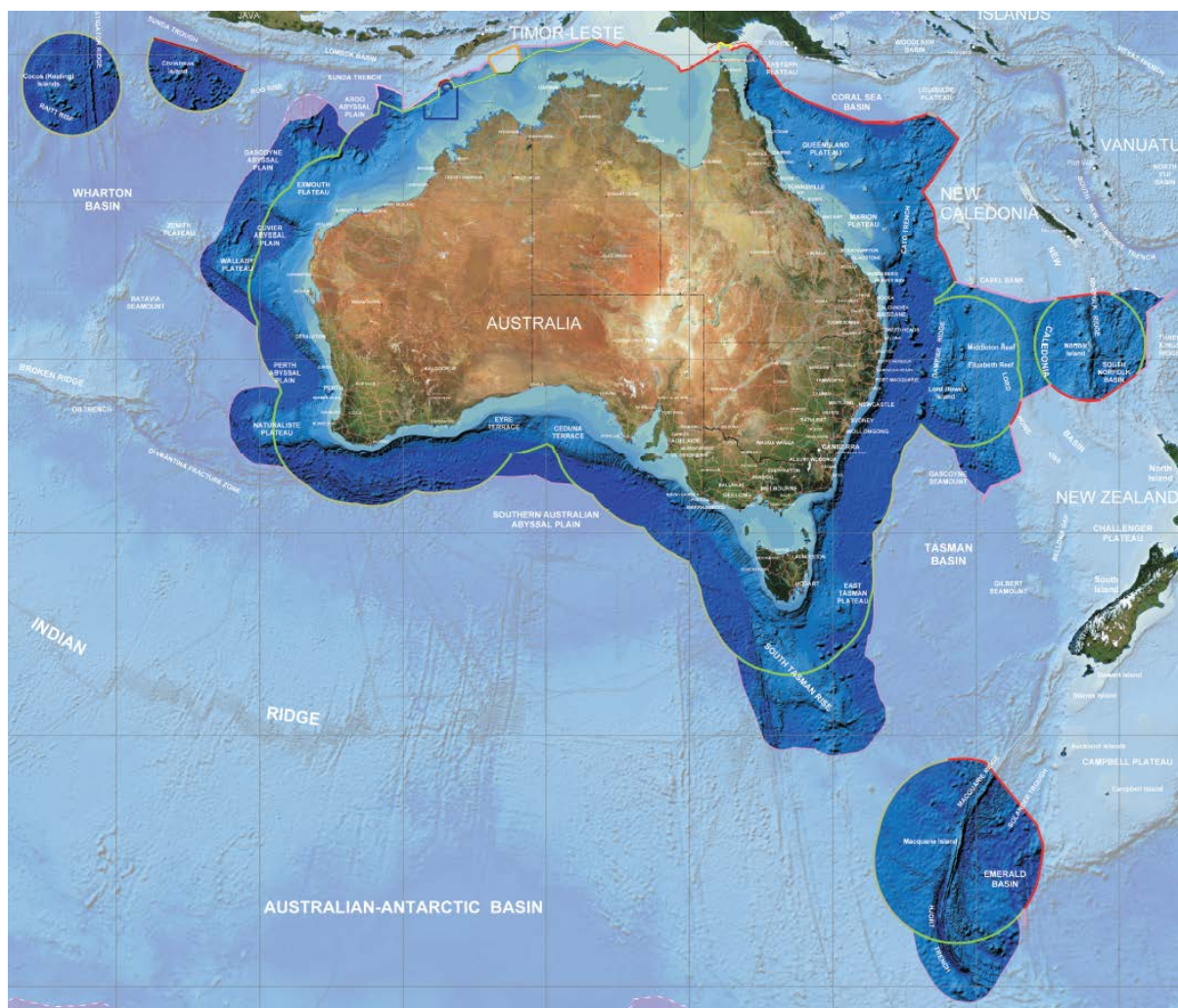
Figure 1-3: The area shown in dark blue is the GDA94 extent. The colours of the lines represent different types of jurisdictional boundaries or proposed jurisdictional boundaries. For more information on the type of boundary, please refer to http://www.ga.gov.au/metadata-gateway/metadata/record/gcat_70362 .
