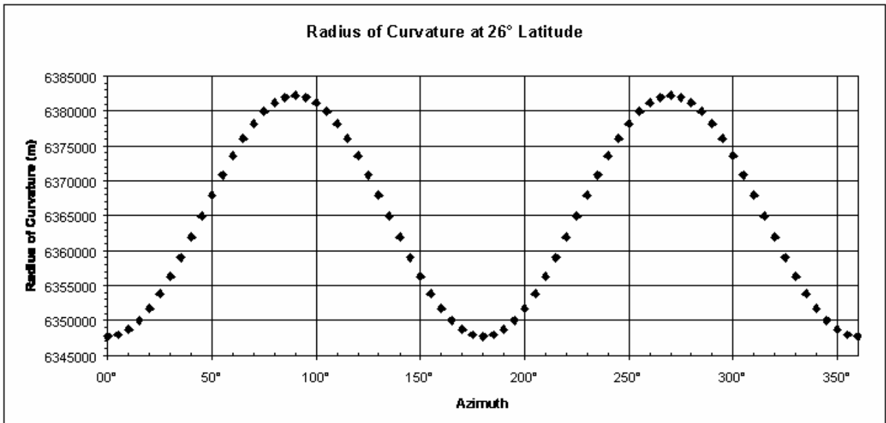
Figure 2-2: Radius of Curvature for Latitude 26°
