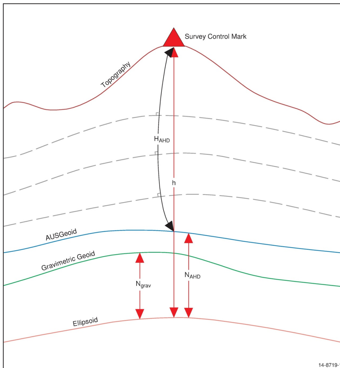
Figure 9-1: Relationship between the ellipsoid, gravimetric geoid, AUSGeoid, and the topography.
