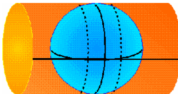
Figure 1-5: Transverse Mercator projection
