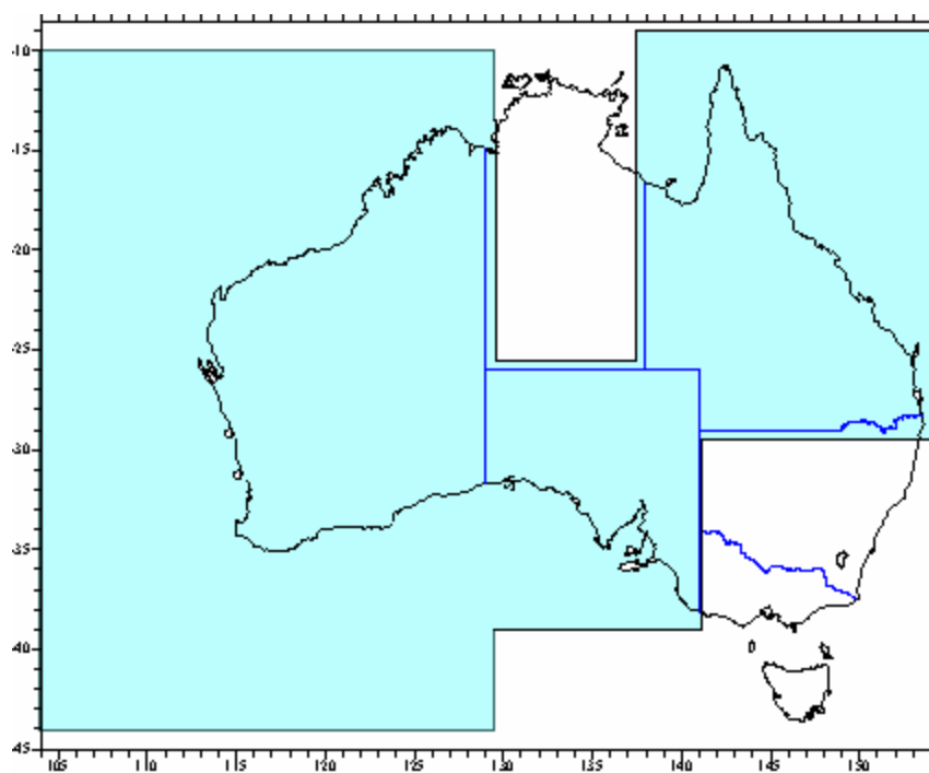
Figure 7-2 AGD 84 to GDA94 Transformation
