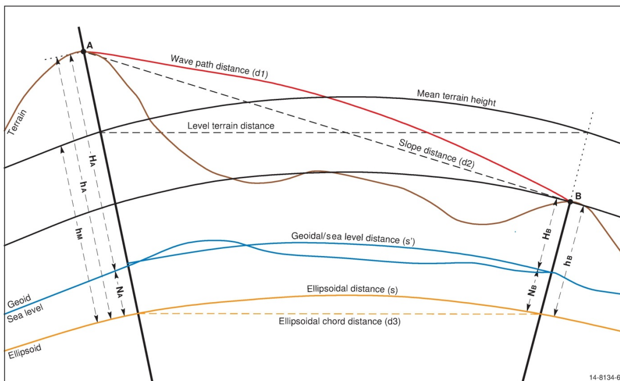
Figure 2-1: Reduction of distance to the Ellipsoid
