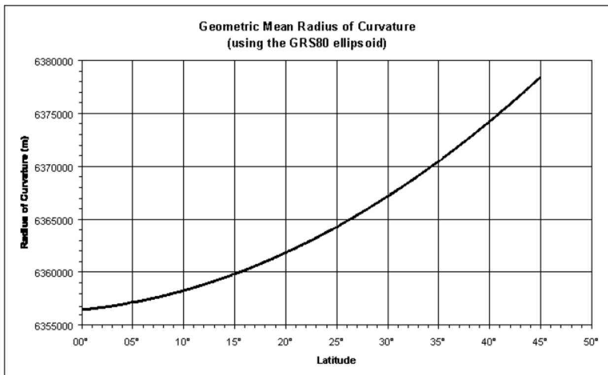
Figure 2-3: Radius of Curvature
